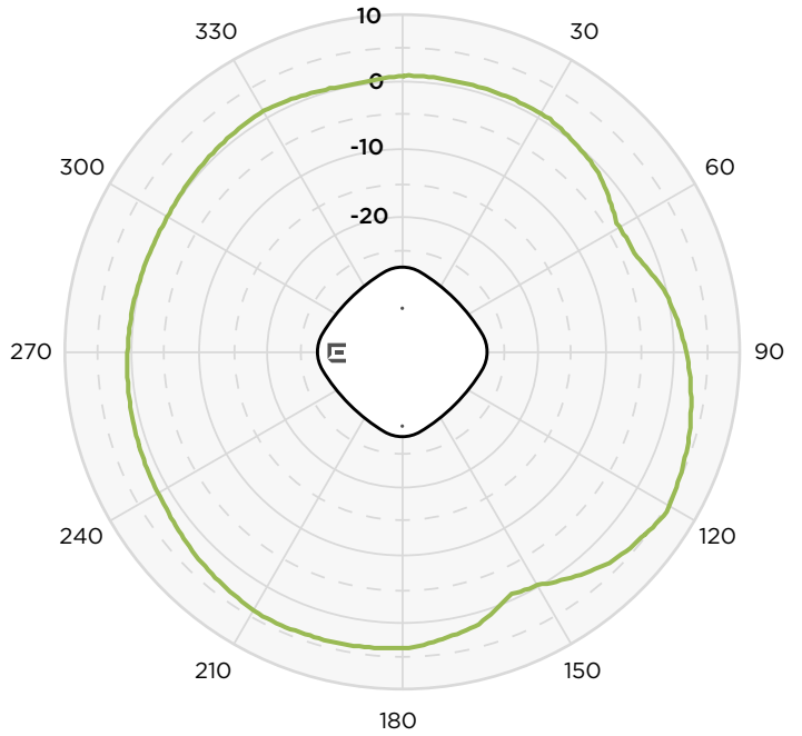
5G Azimuth
