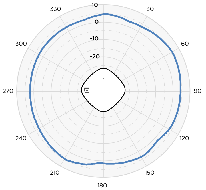
2G Azimuth
